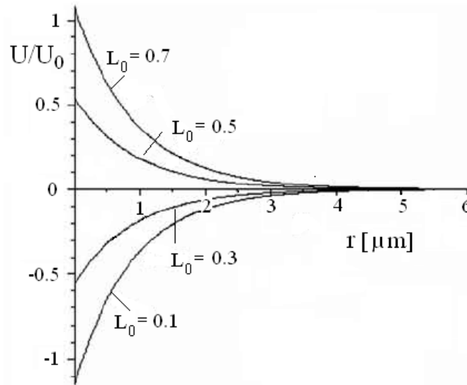
Fig. 1. Profiles of U/U_0 for different L_0 .
