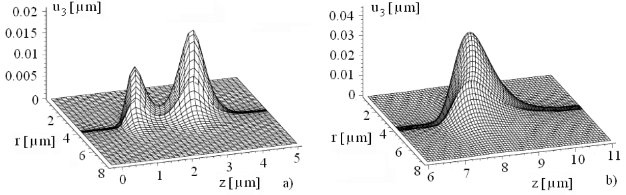
Fig. 2. Profile of u_3 before (a) and after focusing (b).
